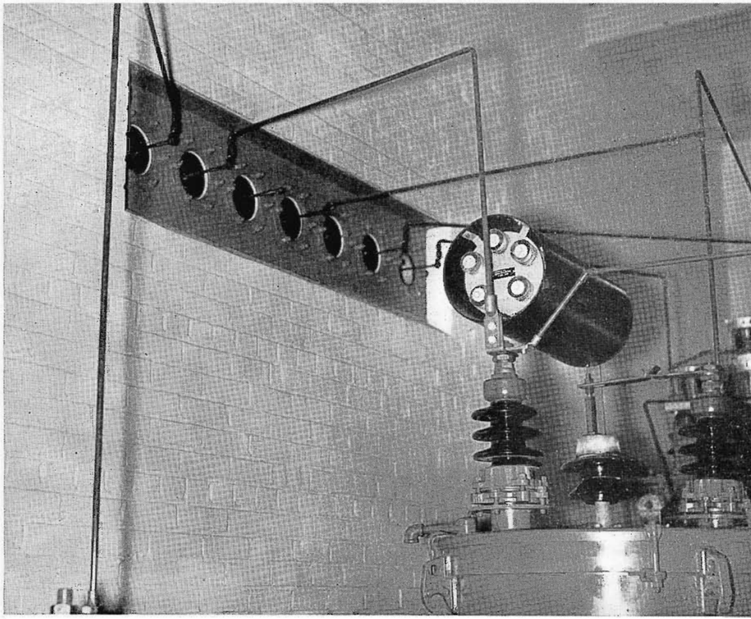
FIG. 5 (left). Specially constructed metal plate with bowl insulators mounted. Installed in wall between the transformer vault and transmitter room.
