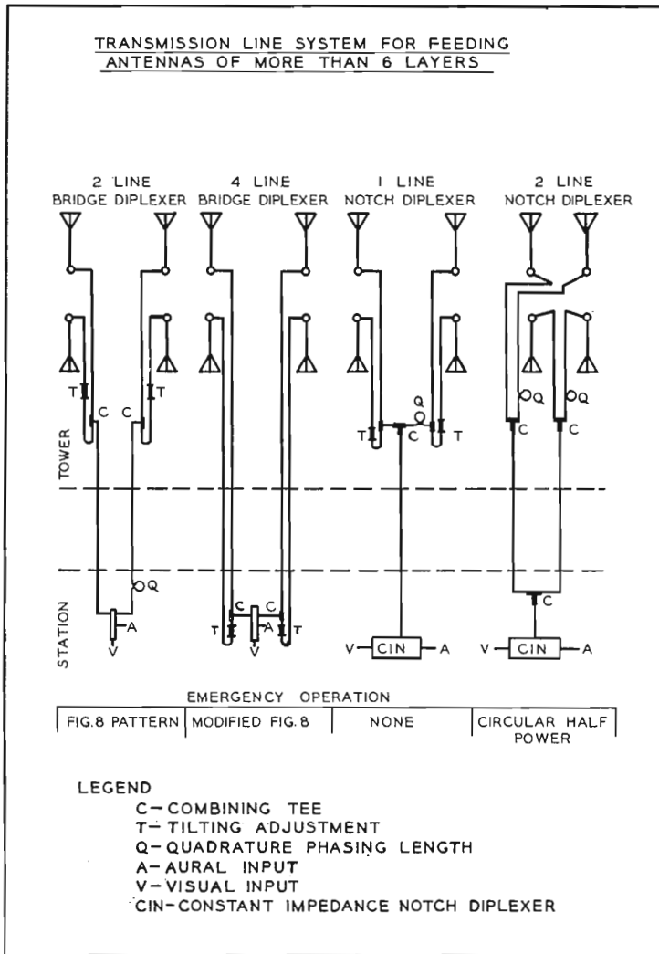
FIG. 3. Chart showing versatility of transmission line systems available with 12-Section Antennas.
