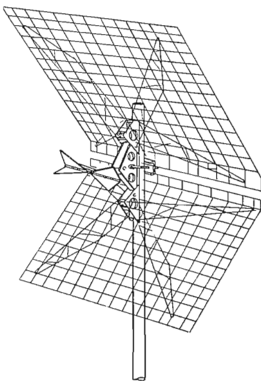
FIG. 7 (left). This is a "corner reflector" antenna of the type used on the truck. This antenna, which has a gain of 9 db at 550 megacycles is used by the RCA Service Company in "difficult" installations.
