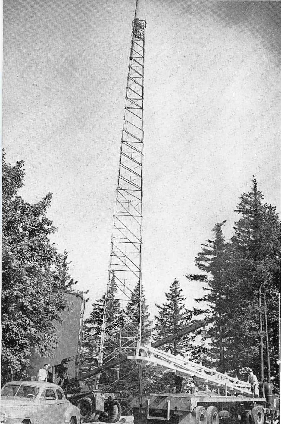
FIG. 1. Unloading the RCA TFU-21B Antenna at KPTV. Because it has no protruding elements the RCA UHF Pylon is easily crated and shipped as a complete unit.
