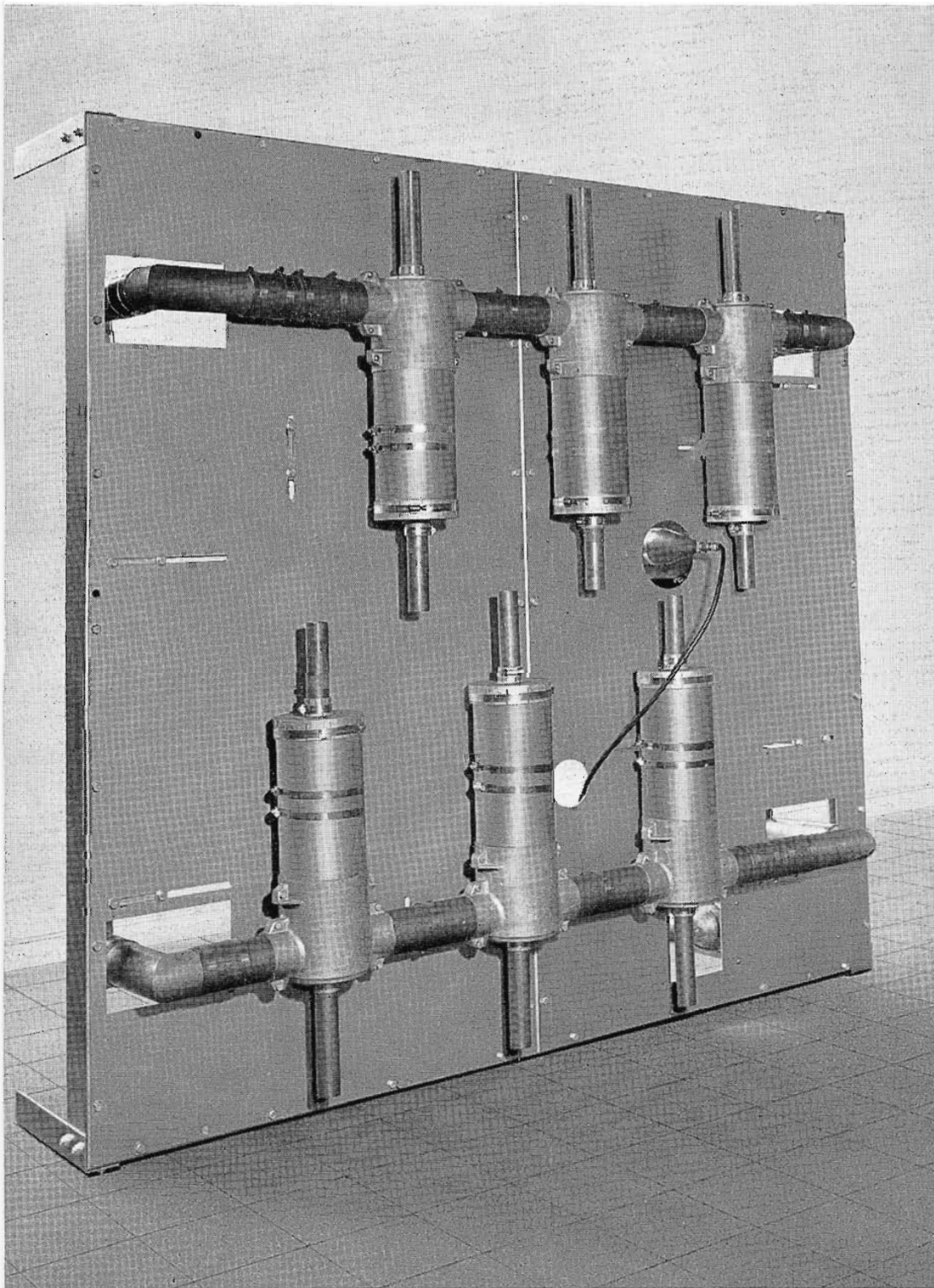
FIG. 9. The Filterplexer can mount either from the overhead or against the wall.
