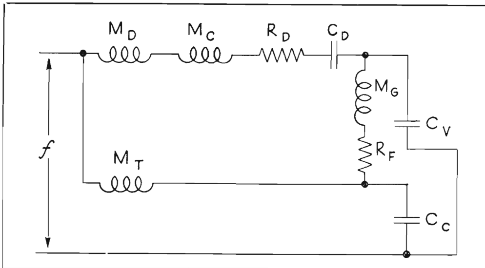
FIG. 4. Electrical analogue of Type BK-1A Microphone.
