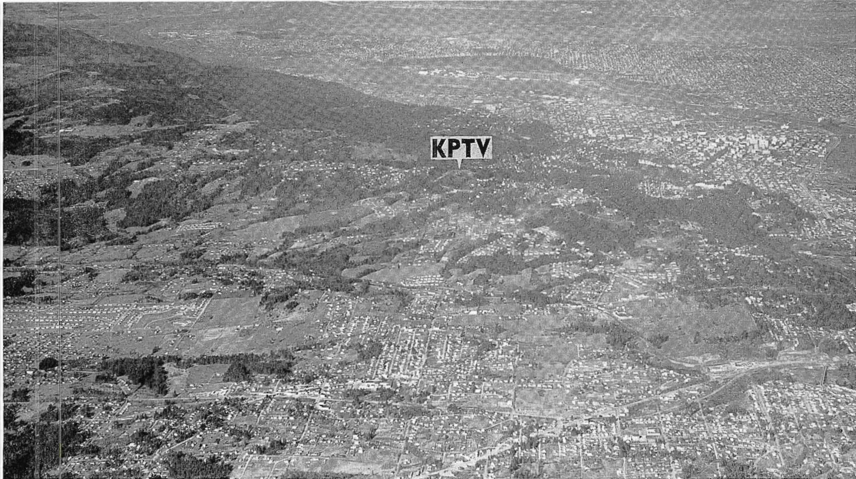
FIG. 2. This aerial view shows the favorable location of KPTV's transmitter. The 1000-foot ridge on which it is located is only two miles from the main business district of the city, which is in the upper right corner of this picture. The fact that the KPTV antenna can be seen from the roof of almost every house in Portland is a great advantage.
