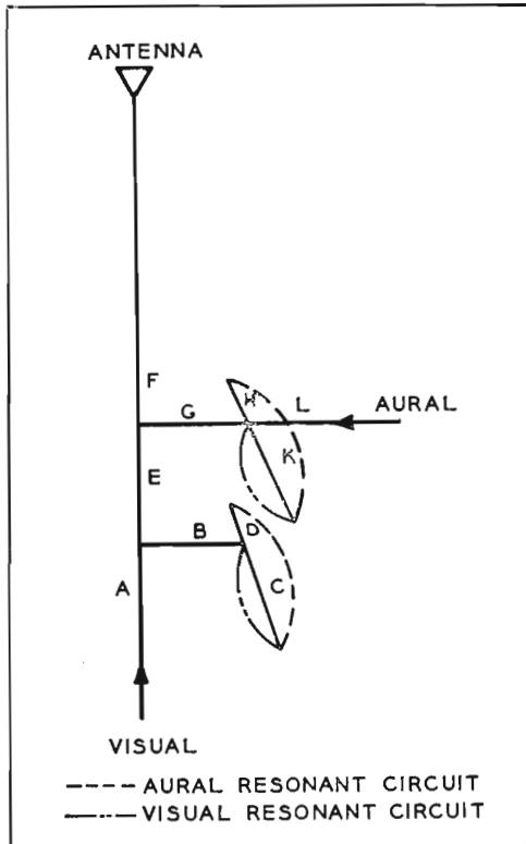
FIG. 3. Notch diplexing circuit. At aural frequency, lines G, H, K, B, D, C, etc., form matched circuit from aural input to antenna with visual input short-circuited to prevent loss of aural energy into visual transmitter. At visual frequency band (except at 4.5 mc above visual carrier), these same lines form matched circuit from visual input to antenna with aural input short circuited. Thus visual characteristic is constant except for notch at 4.5 mcs in attenuation vs. frequency characteristic.
