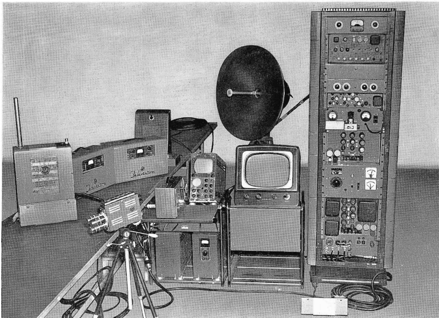
FIG. 14. View of the overall equipment which comprises a complete "Walkie-Lookie" system.
