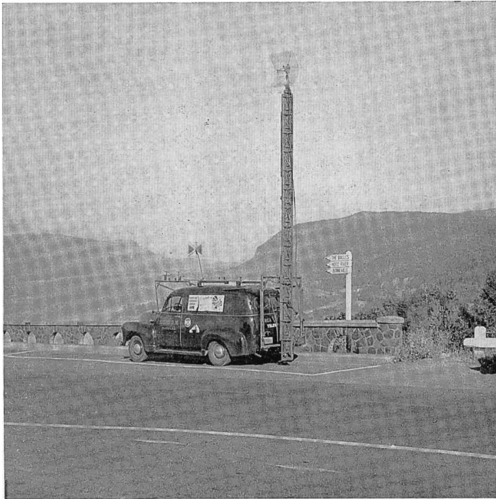
FIG. 5 (left). This is the RCA Service Company's field truck which was used in making the observations on which this report is based. The antenna on the extension tower can be raised to any desired height between 20 feet and 70 feet. For field intensity measurements this antenna was connected to a Stoddard Field Intensity Meter mounted at the observer's position in the truck. The bow tie antenna near the front of the truck was connected to an RCA U-70 Selector feeding into an RCA 630 TV Receiver. Both receiver and field intensity meter were supplied 110 volt power by a small gas engine generator in the truck and could be operated with the truck in motion. The equipment for this field truck was planned and installed by J. D. Callaghan and A. I. Kothe of the Engineering Section of the RCA Service Company. The truck is a part of the permanent equipment of the RCA Service Company's Portland branch. It will be used by technicians in determining the best locations for difficult antenna installations.
