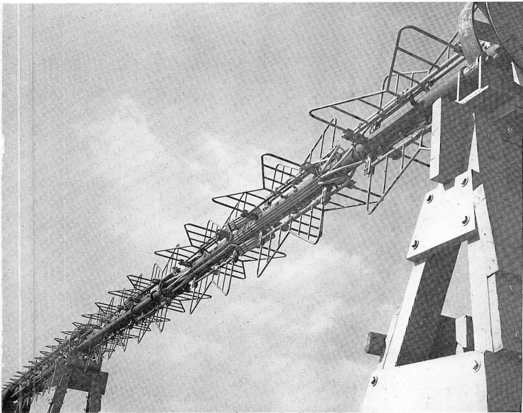
FIG. 2. View of the new 12-Section VHF Antenna, Type TF-12AH for high-band operation. This setup permits field measurements of both power gain and coverage patterns.
