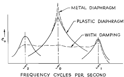
FIG. 5. Theoretical response characteristics of Type BK-1A Microphone.
