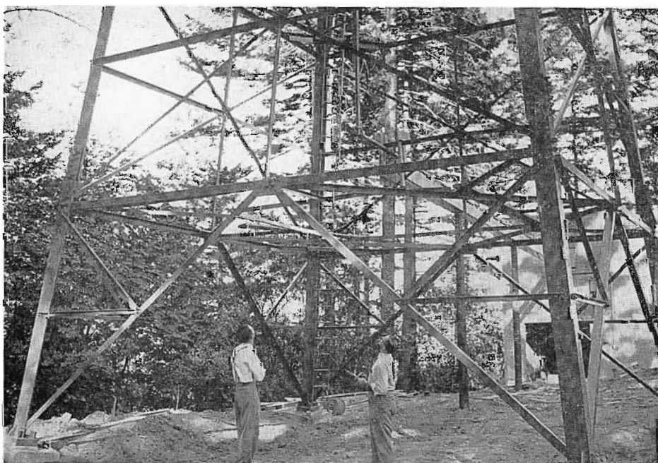
FIG. 6 (below). View of the base of the tower showing the single 3\frac{1}{8} -inch coaxial line which feeds power from the transmitter to the antenna.
