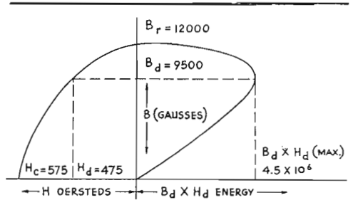
FIG. 8. Magnetization curve for Alnico V, Type BK-1A Microphone.
