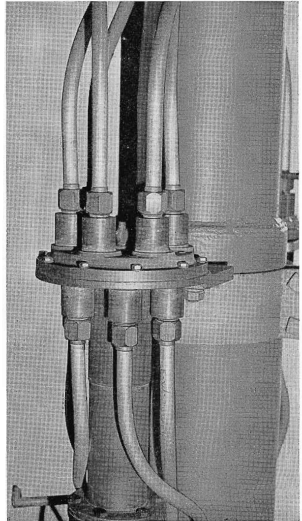
FIG. 4. Power enters above the junction box through 3 1/2-inch transmission line and connects through smaller feedlines to individual radiators.
