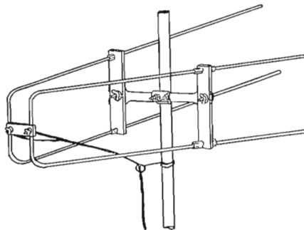
FIG. 6 (above). This "stacked V" antenna is being used for standard installations in the Portland area by the RCA Service Company. It has a gain of 7 db at 550 megacycles, and is reasonably good for VHF as well as UHF.
