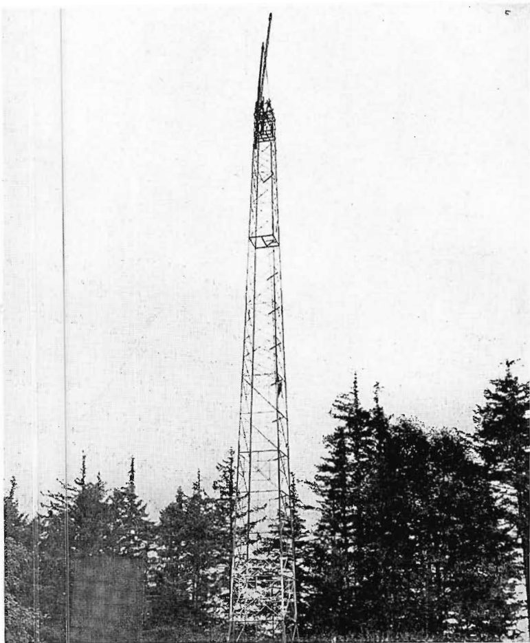
FIG. 4. At the top of the tower a gin pole of reasonable dimensions is used to set the antenna in place. There is nothing to be mounted on the antenna after it is put in place.
