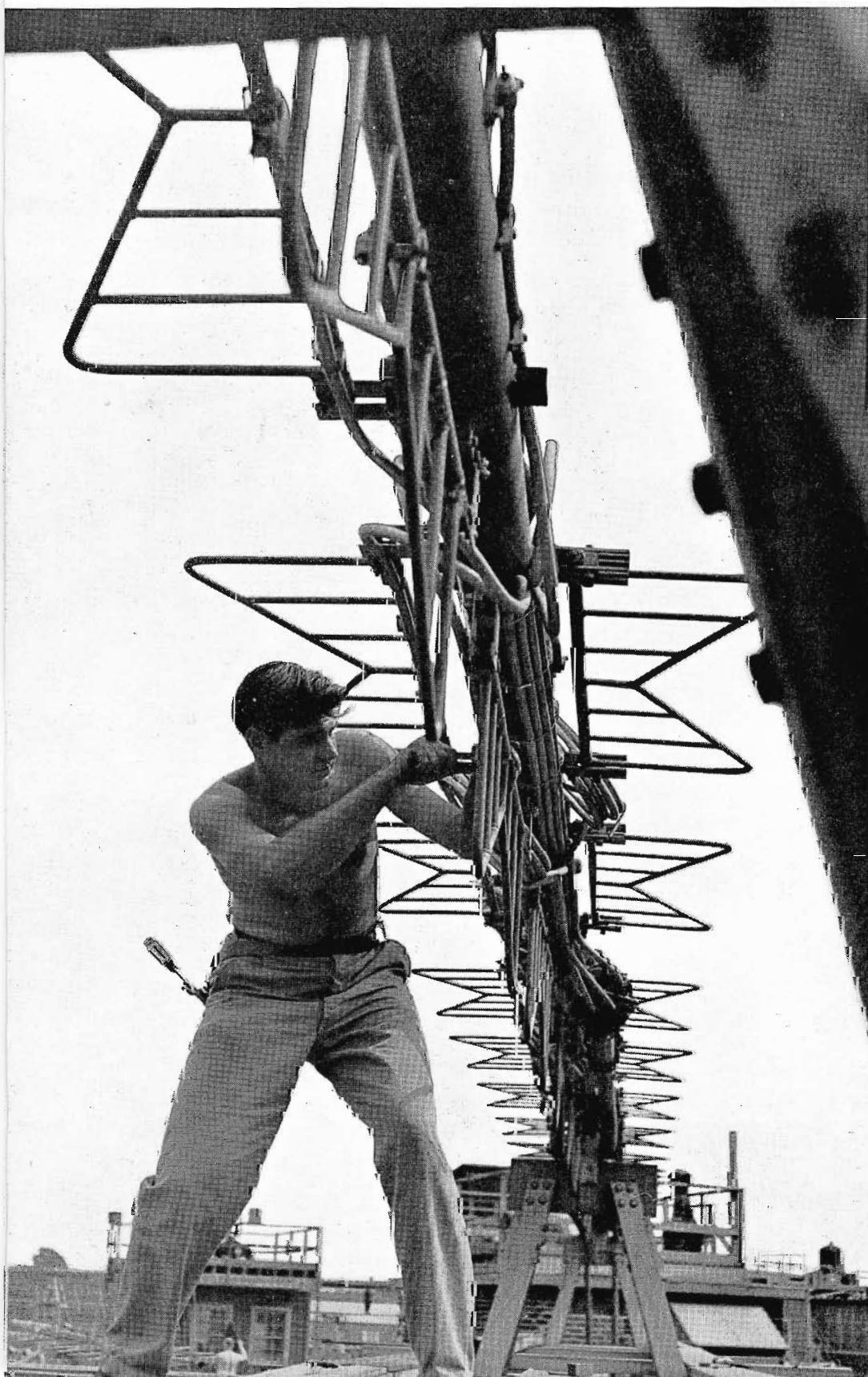
FIG. 1. B. T. Bailey of RCA's Engineering Products Department, shown adjusting a batwing element on RCA's new 12-Section Superturnstile Antenna.
