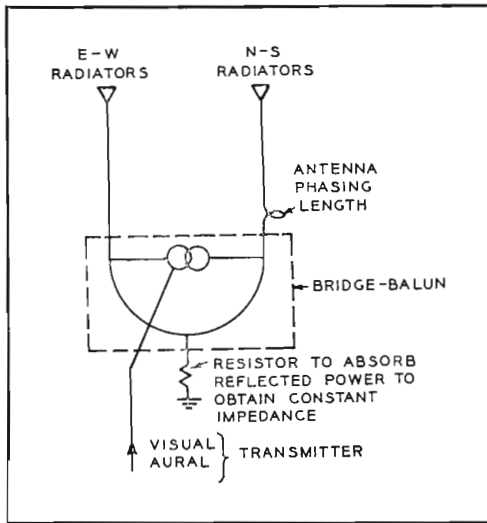
FIG. 5. Power equalizer circuit is used to obtain improved bandwidth for antennas that otherwise have a relatively poor impedance characteristics. The bridge-balun is equivalent to bridge circuit.
