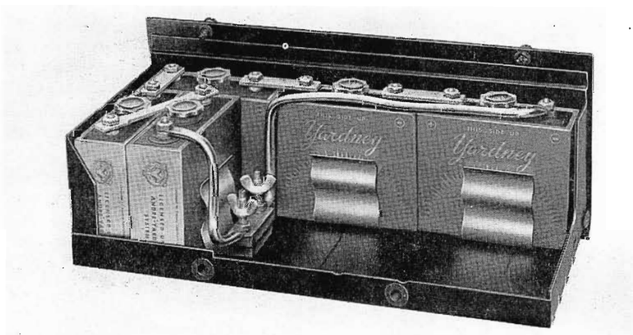
FIG. 8. Below is a view of the battery drawer assembly, complete with a set of the batteries required for use.
