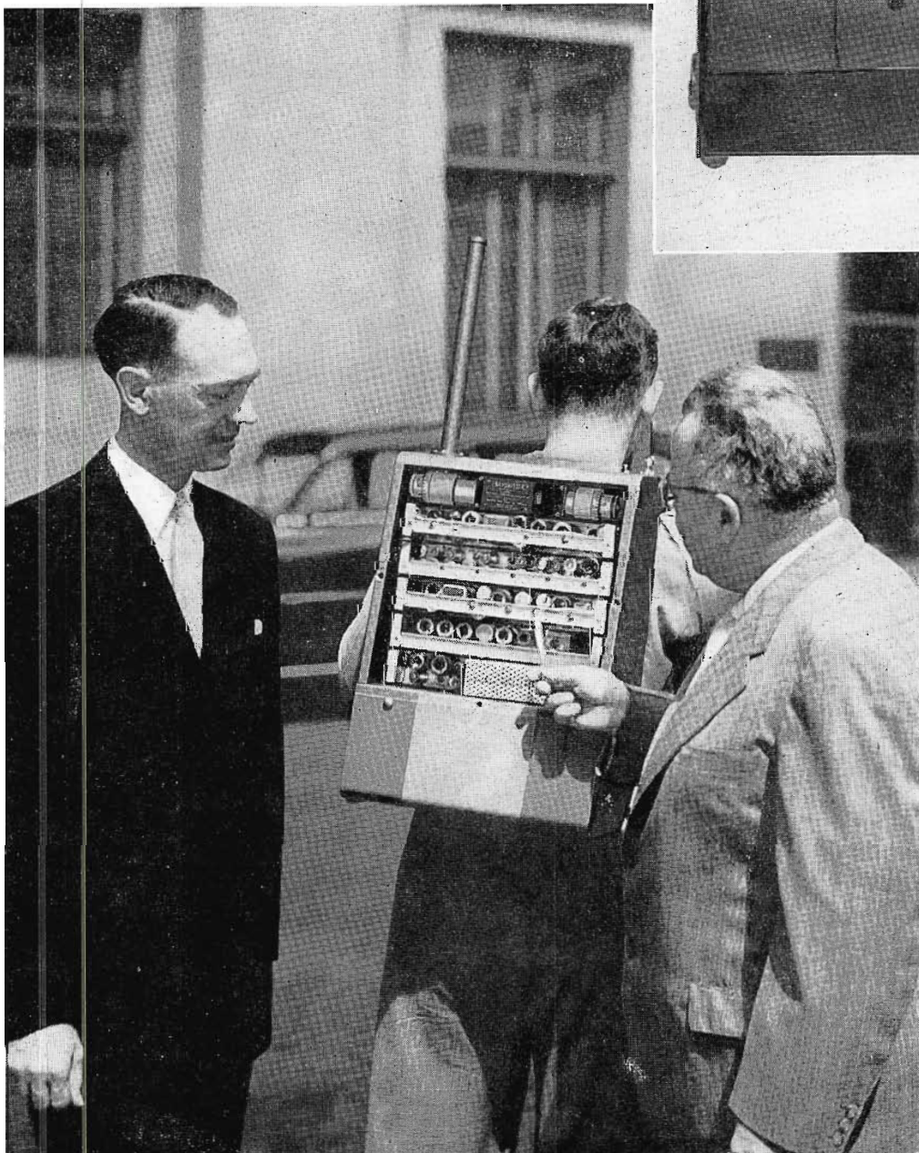
FIG. 10. Closeup of the "Walkie-Lookie" Pack Unit showing the various "plug-in" chassis arrangement used.
